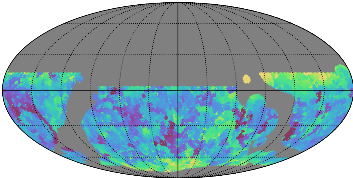
baseline_v3.5_10yrs WFD g band: Min seeingEff
