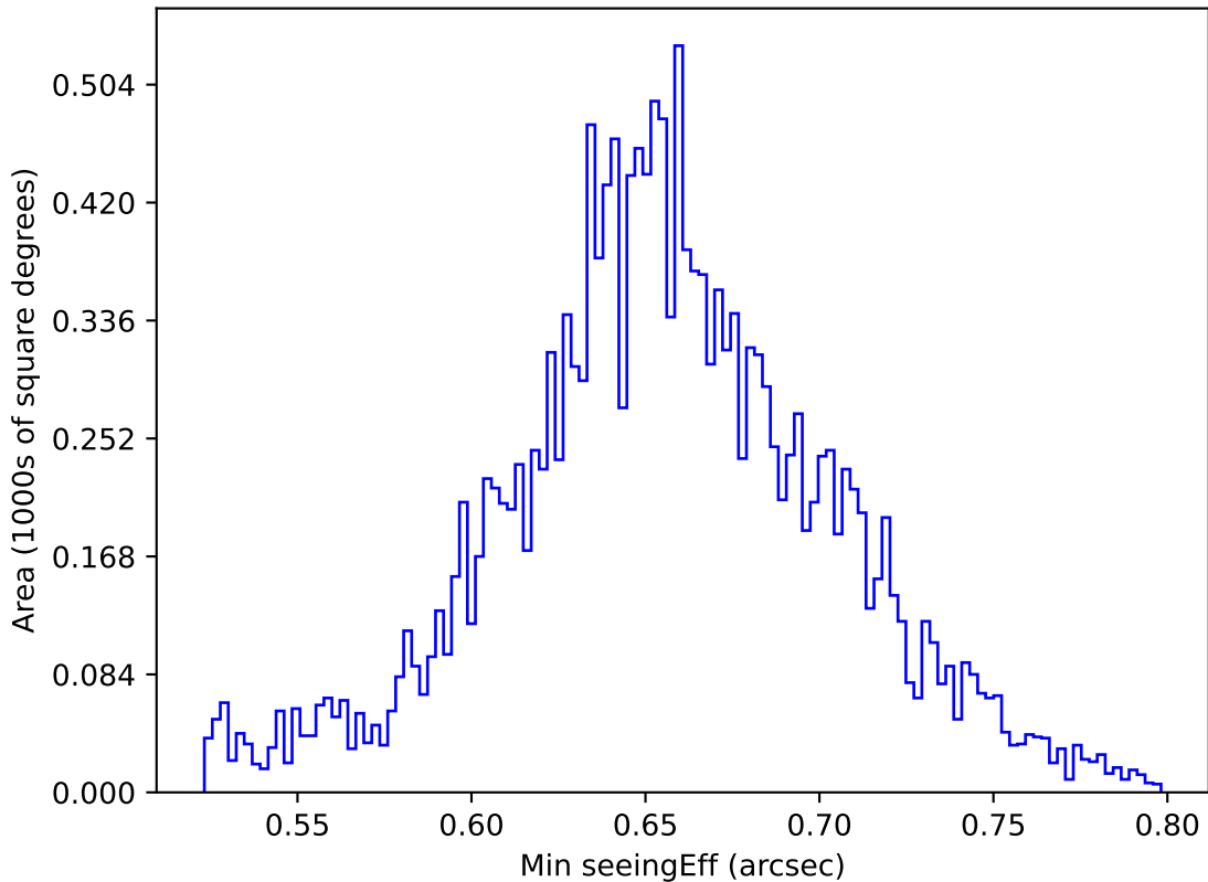
baseline_v3.5_10yrs WFD g band: Min seeingEff
