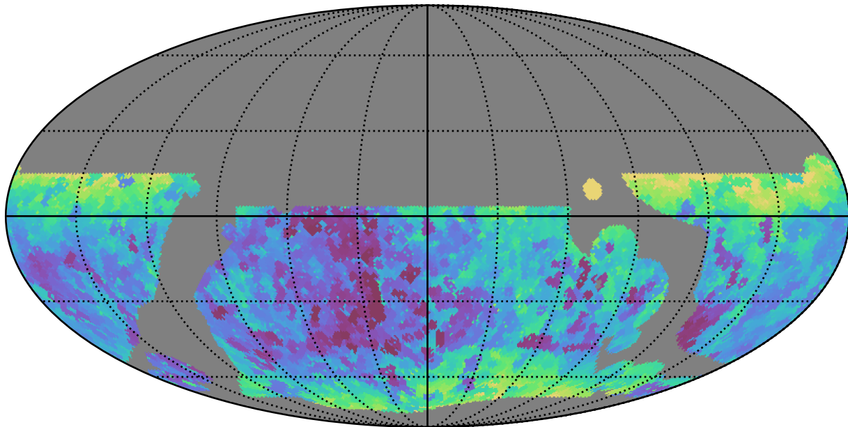
baseline_v3.5_10yrs WFD all bands: Min seeingEff
