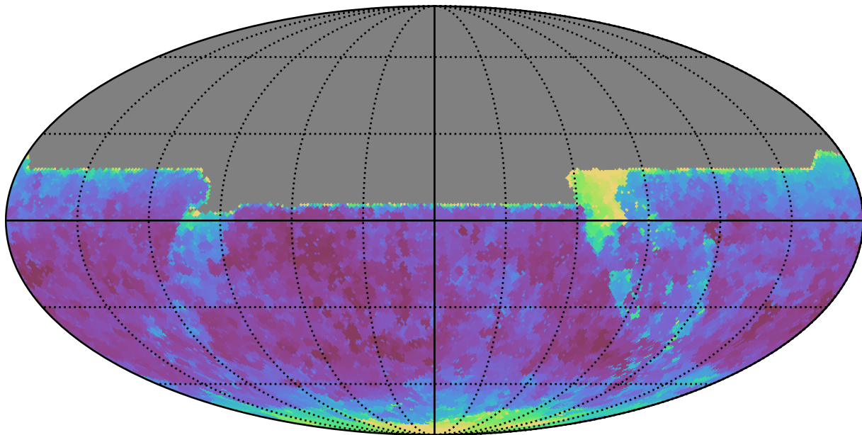
baseline_v3.5_10yrs All sky y band: Min seeingEff
