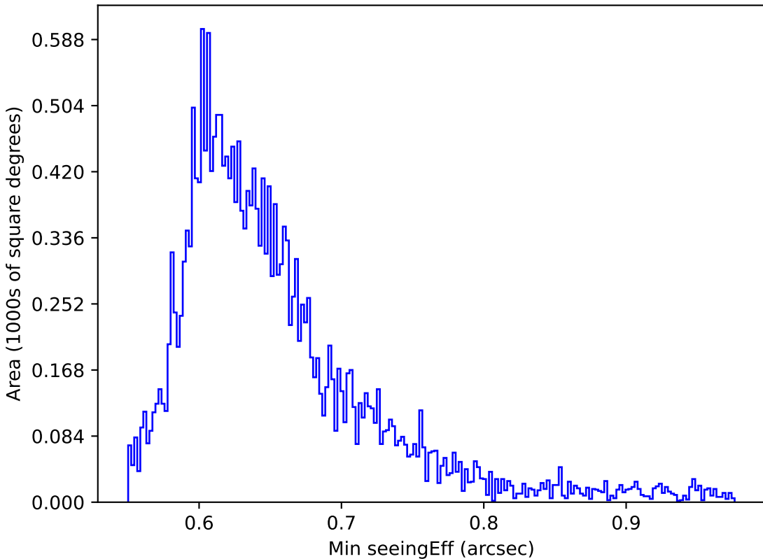
baseline_v3.5_10yrs All sky y band: Min seeingEff
