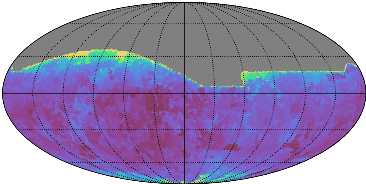
baseline_v3.5_10yrs All sky r band: Min seeingEff
