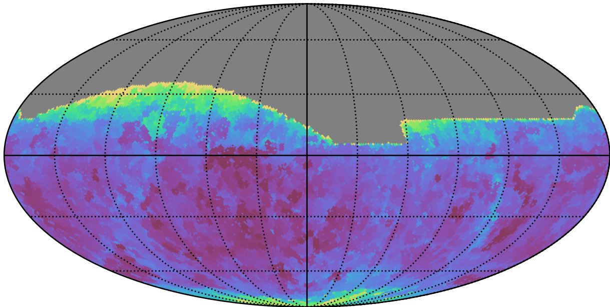
baseline_v3.5_10yrs All sky i band: Min seeingEff
