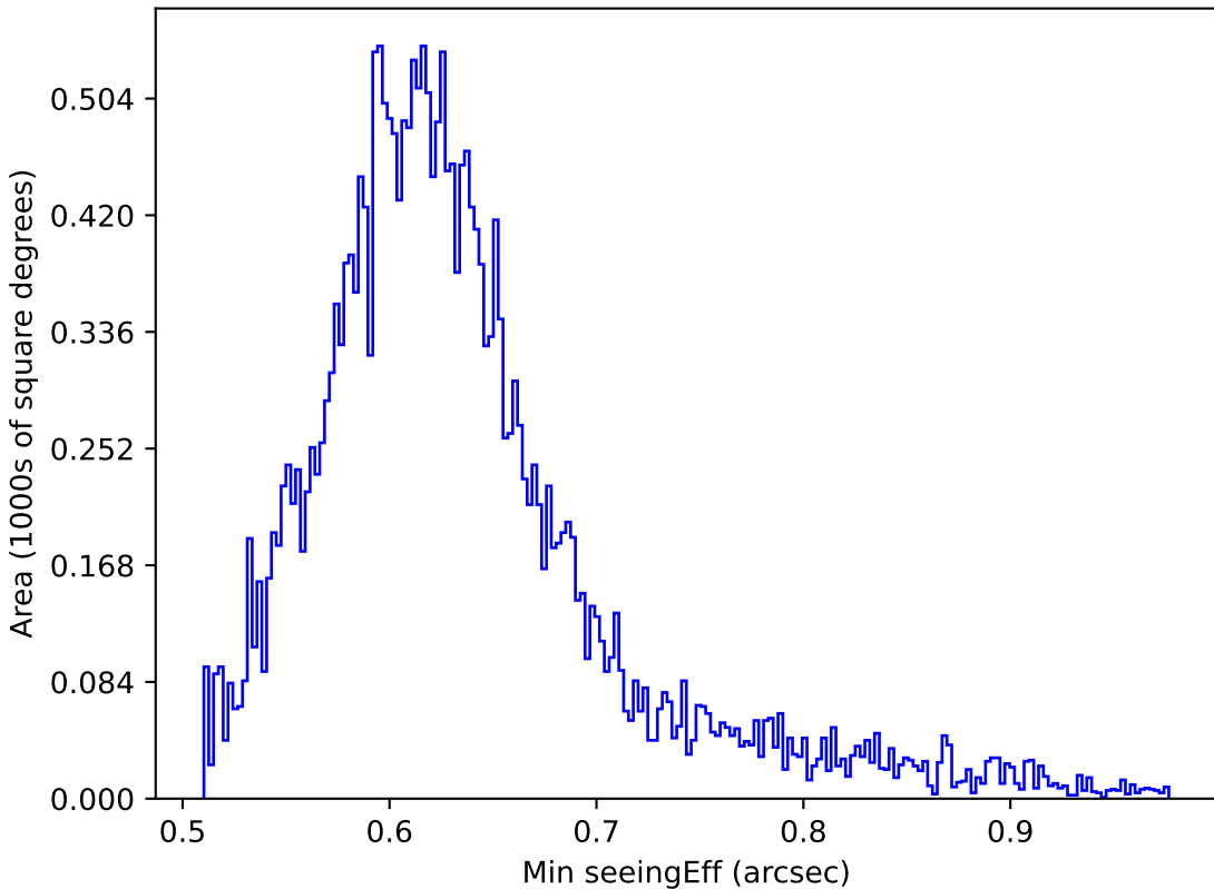
baseline_v3.5_10yrs All sky i band: Min seeingEff
