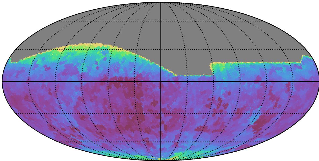
baseline_v3.5_10yrs All sky all bands: Min seeingEff
