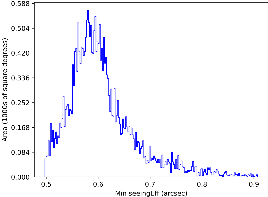
baseline_v3.5_10yrs All sky all bands: Min seeingEff
