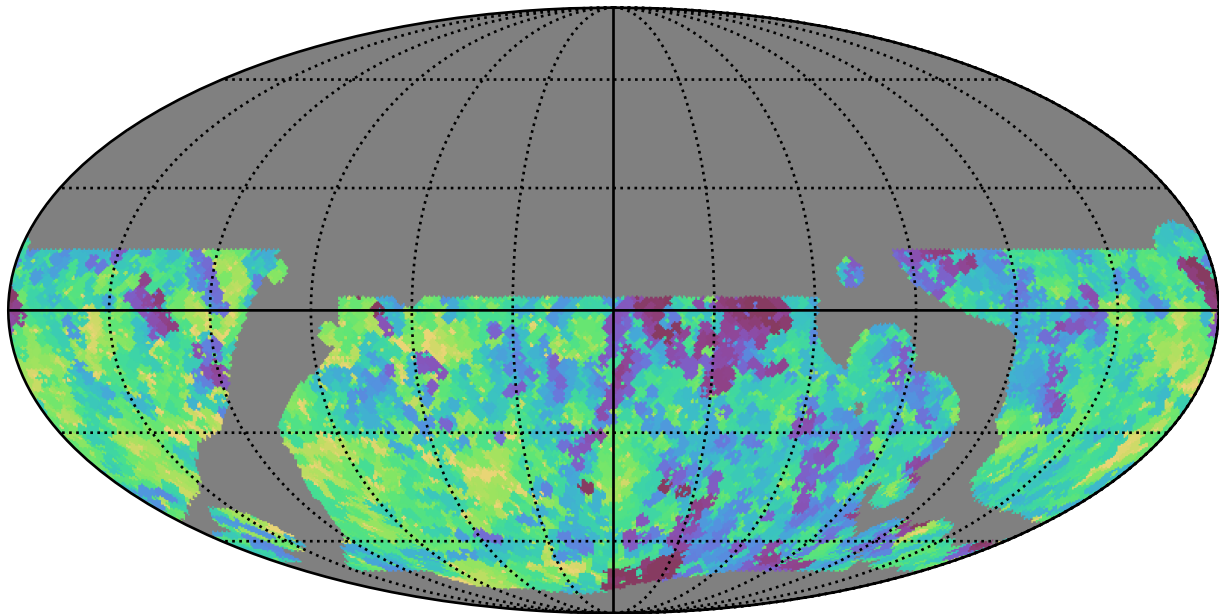
baseline_v3.5_10yrs WFD z band: Min saturation_mag
