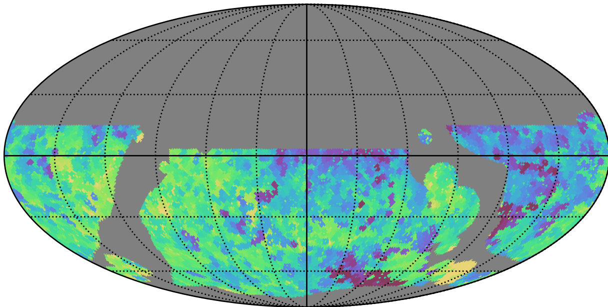
baseline_v3.5_10yrs WFD y band: Min saturation_mag
