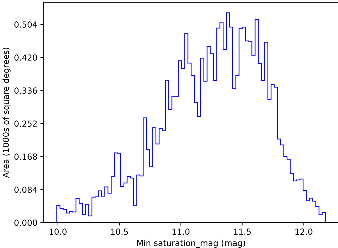
baseline_v3.5_10yrs WFD y band: Min saturation_mag
