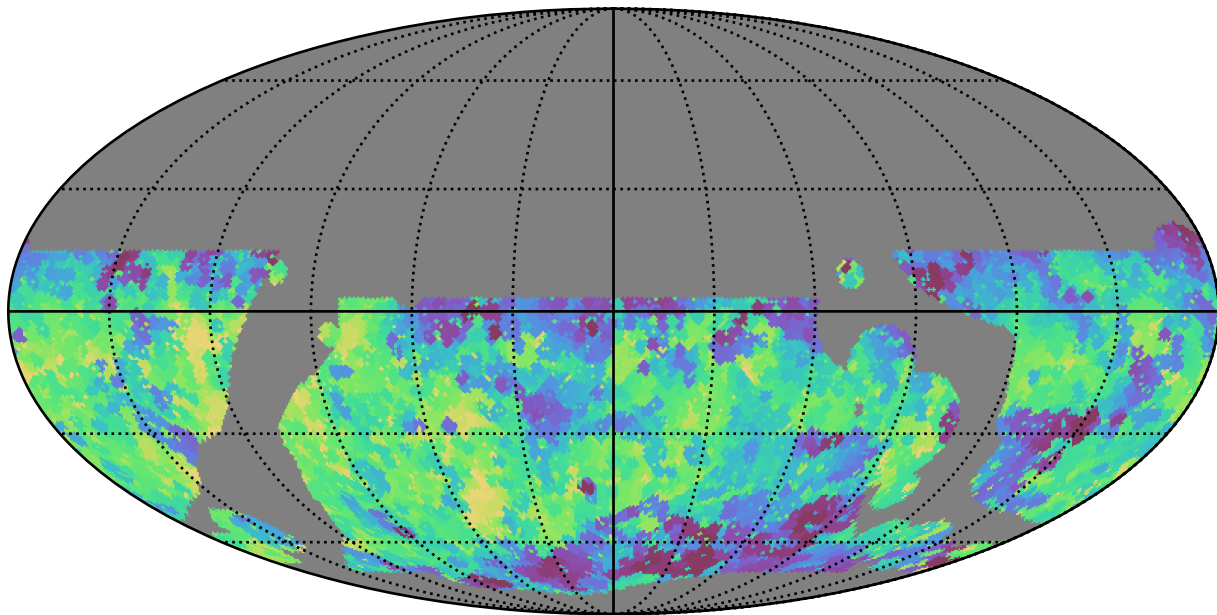
baseline_v3.5_10yrs WFD u band: Min saturation_mag
