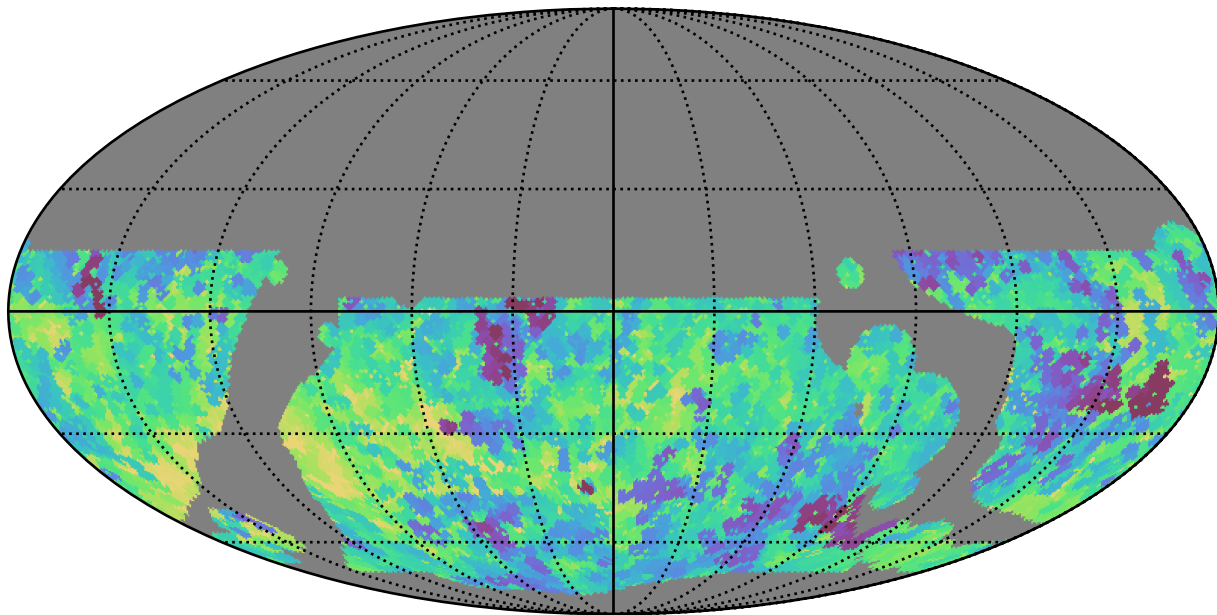
baseline_v3.5_10yrs WFD r band: Min saturation_mag
