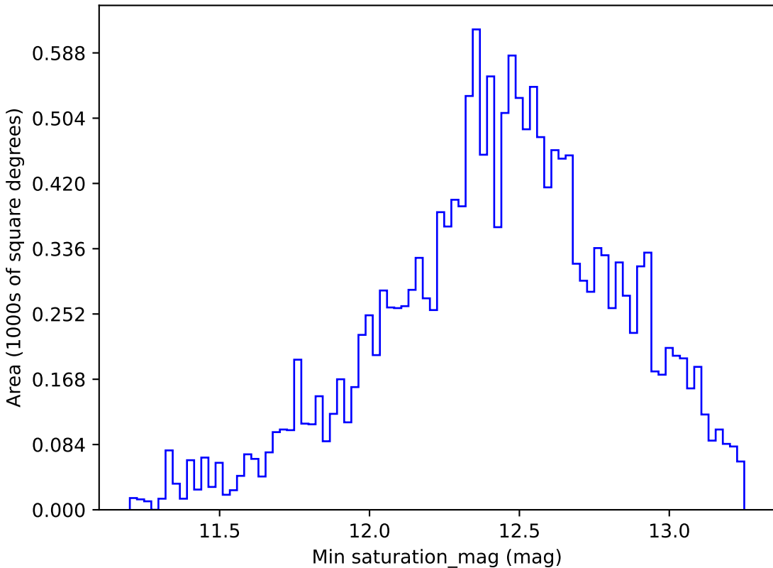
baseline_v3.5_10yrs WFD r band: Min saturation_mag
