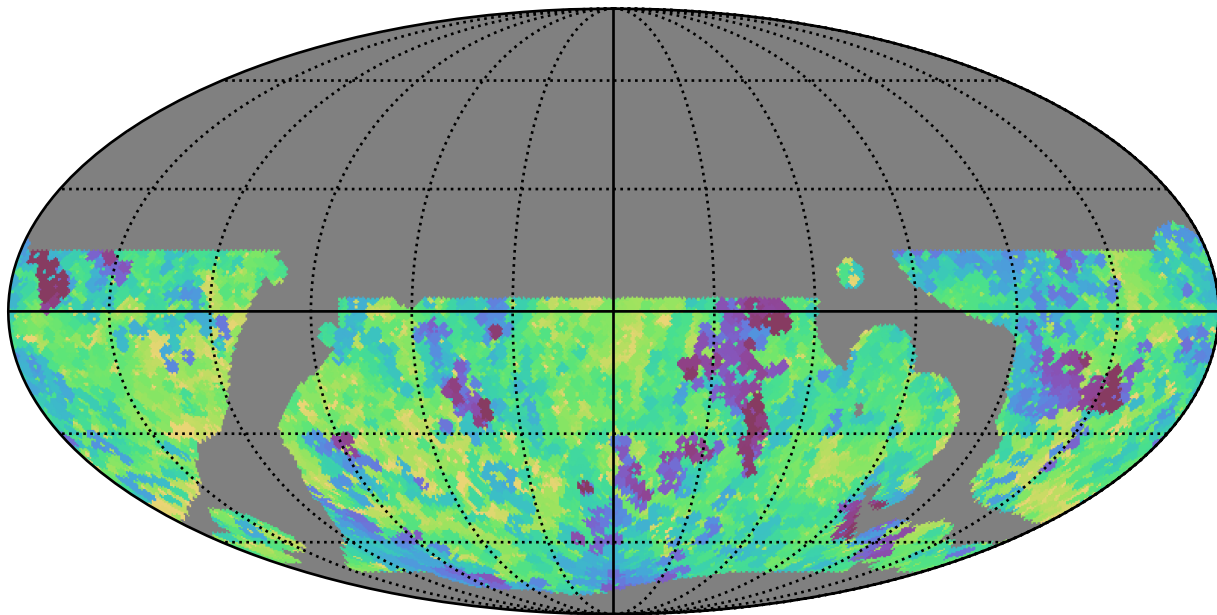
baseline_v3.5_10yrs WFD i band: Min saturation_mag
