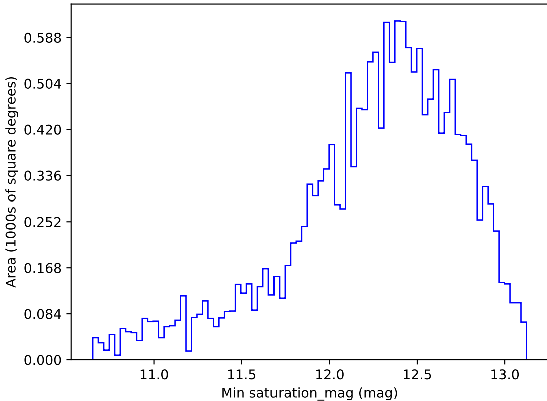
baseline_v3.5_10yrs WFD i band: Min saturation_mag
