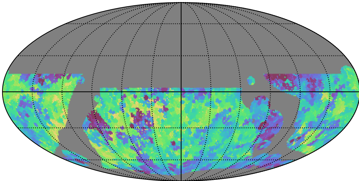
baseline_v3.5_10yrs WFD g band: Min saturation_mag
