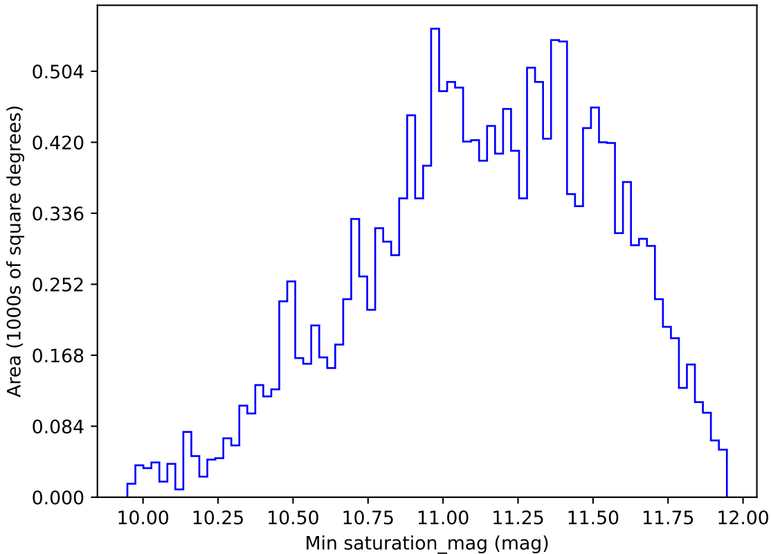
baseline_v3.5_10yrs WFD all bands: Min saturation_mag
