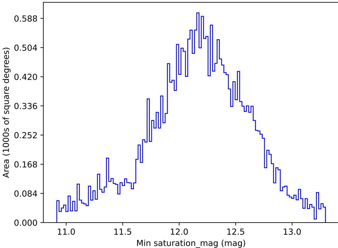
baseline_v3.5_10yrs All sky z band: Min saturation_mag
