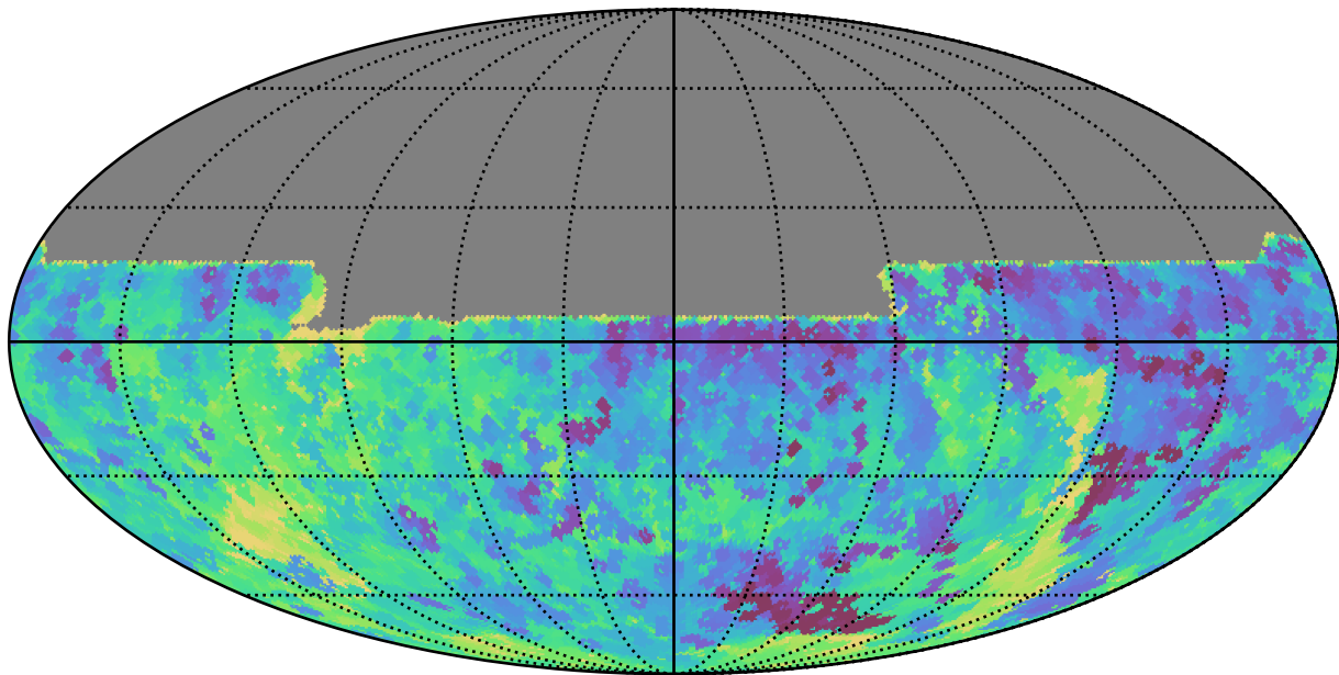
baseline_v3.5_10yrs All sky y band: Min saturation_mag
