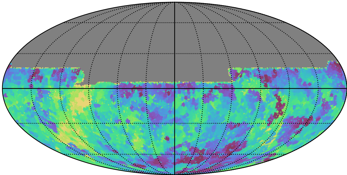
baseline_v3.5_10yrs All sky u band: Min saturation_mag
