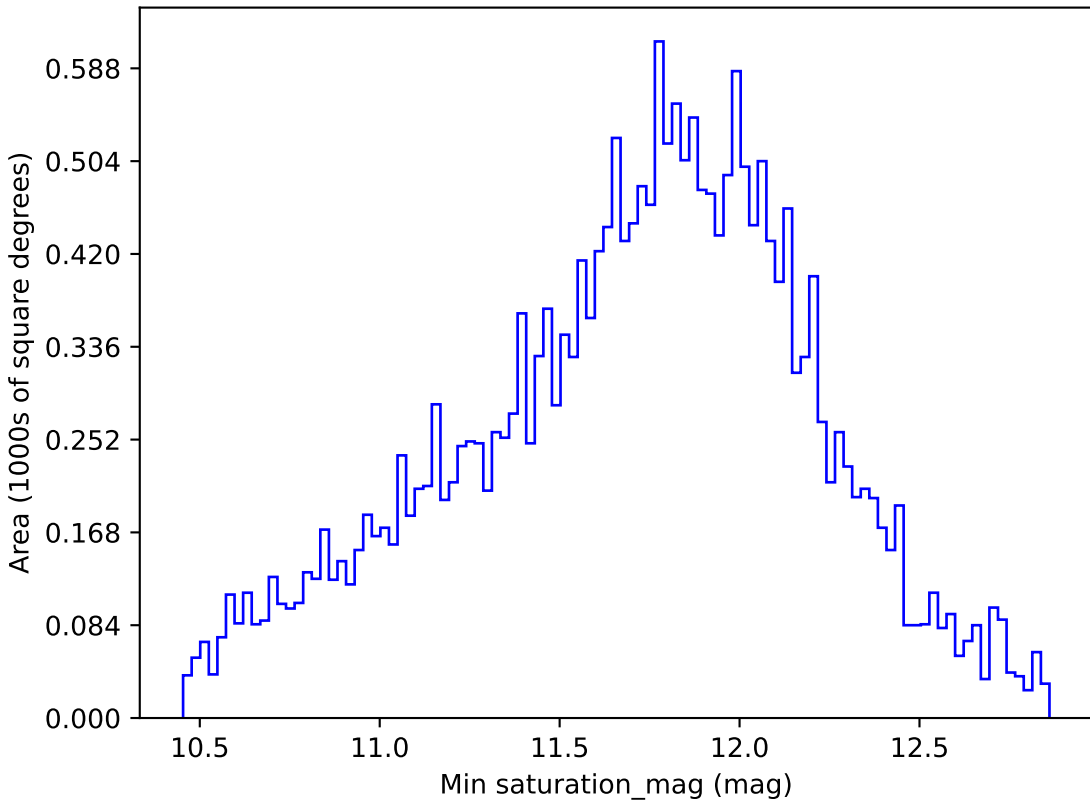
baseline_v3.5_10yrs All sky u band: Min saturation_mag
