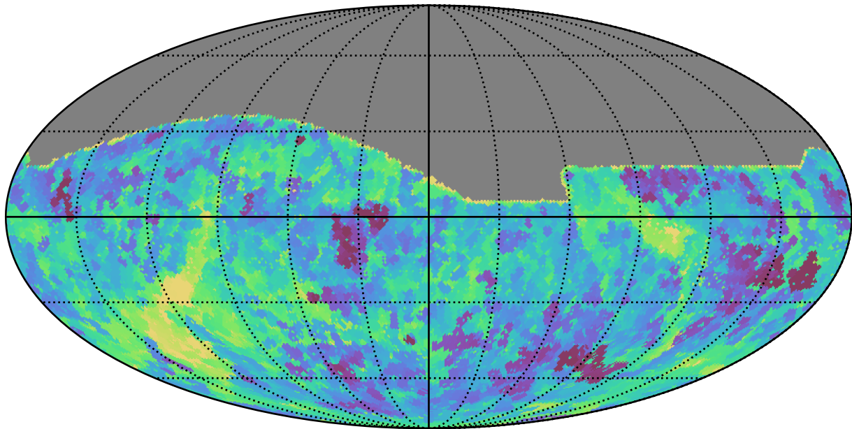
baseline_v3.5_10yrs All sky r band: Min saturation_mag
