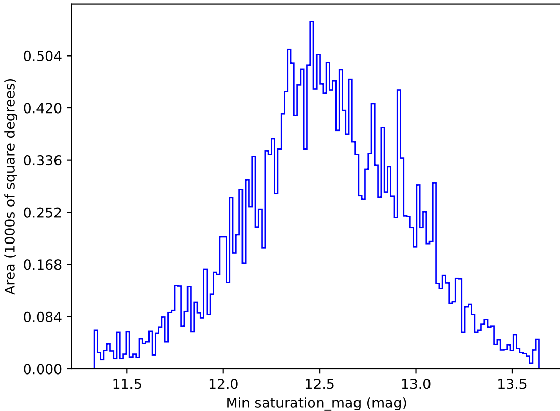
baseline_v3.5_10yrs All sky r band: Min saturation_mag
