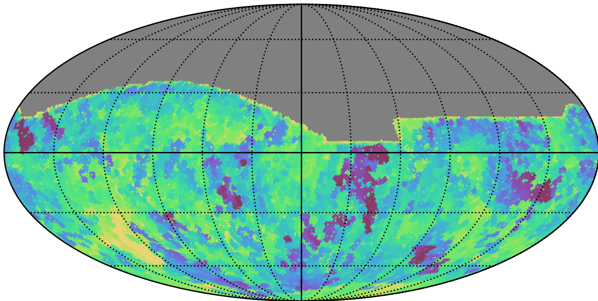
baseline_v3.5_10yrs All sky i band: Min saturation_mag
