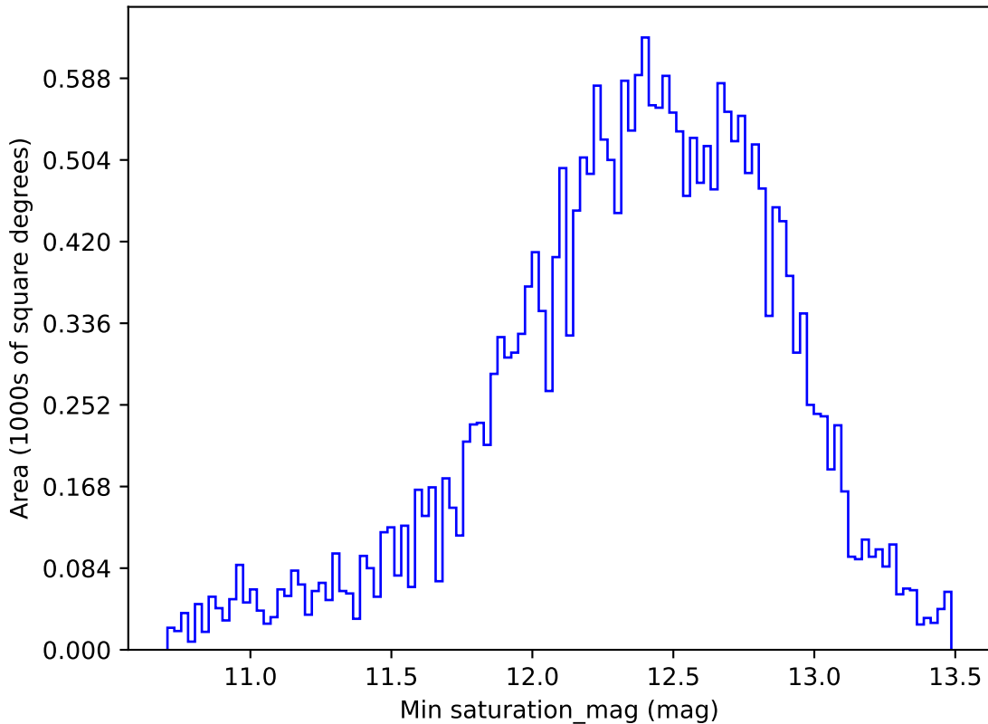
baseline_v3.5_10yrs All sky i band: Min saturation_mag
