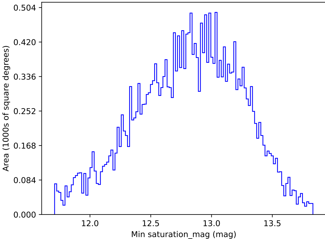
baseline_v3.5_10yrs All sky g band: Min saturation_mag
