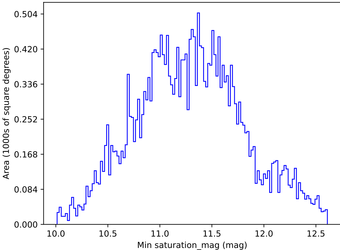
baseline_v3.5_10yrs All sky all bands: Min saturation_mag
