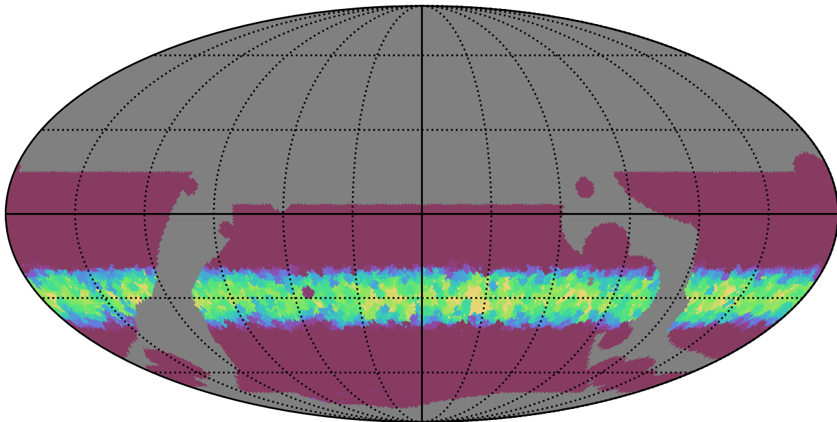
baseline_v3.5_10yrs WFD z band: Min normairmass
