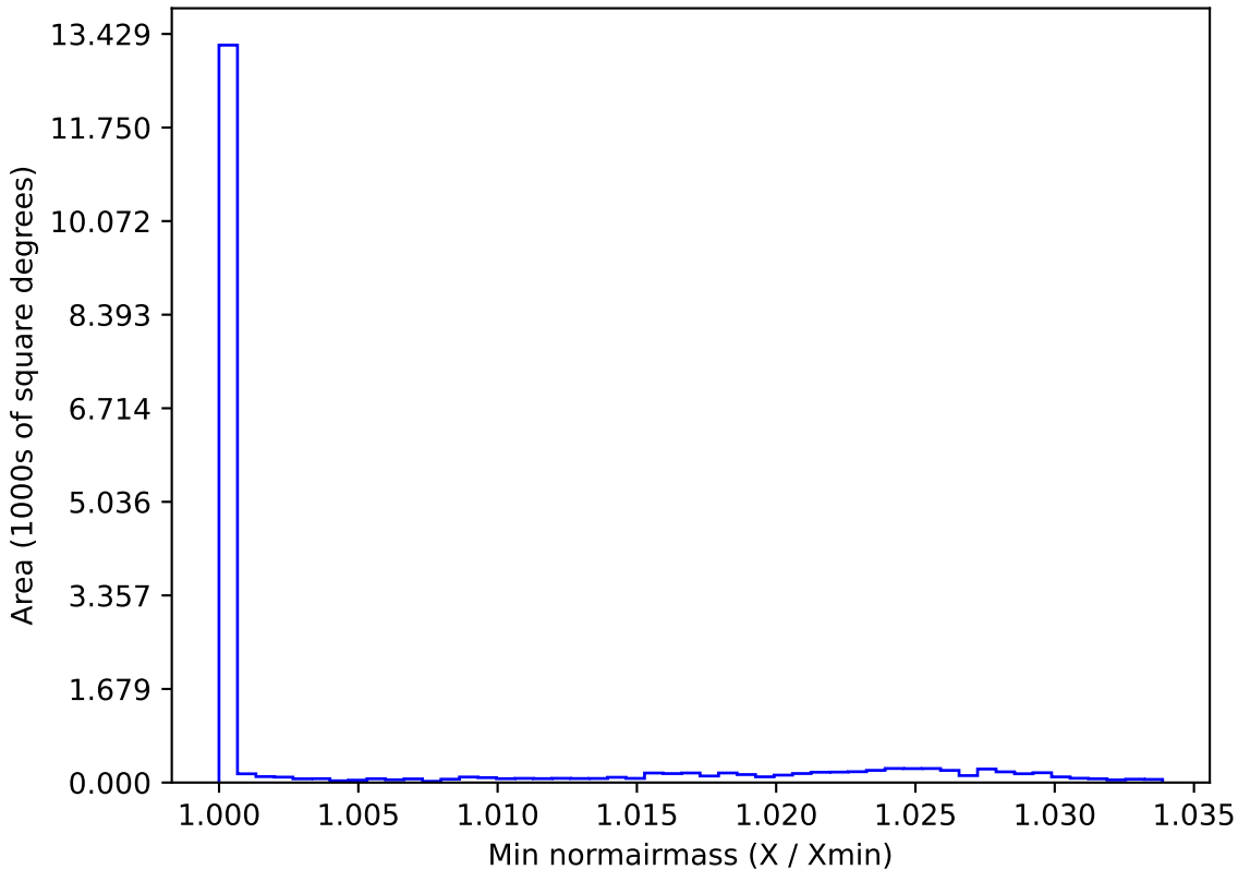
baseline_v3.5_10yrs WFD z band: Min normairmass
