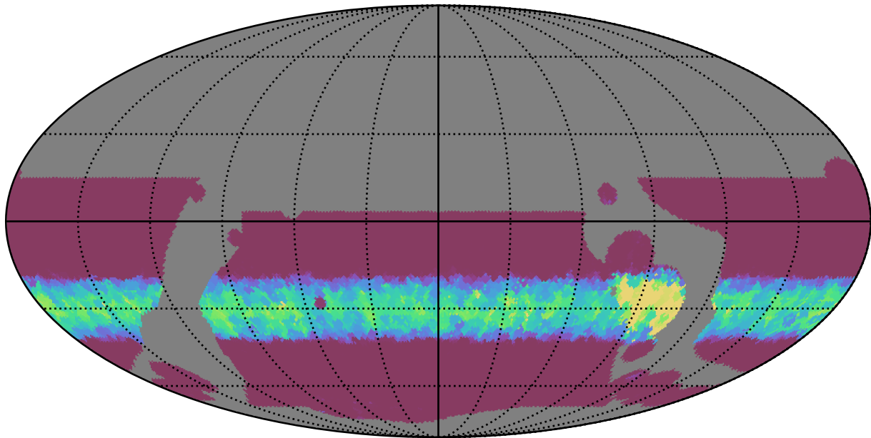
baseline_v3.5_10yrs WFD y band: Min normairmass
