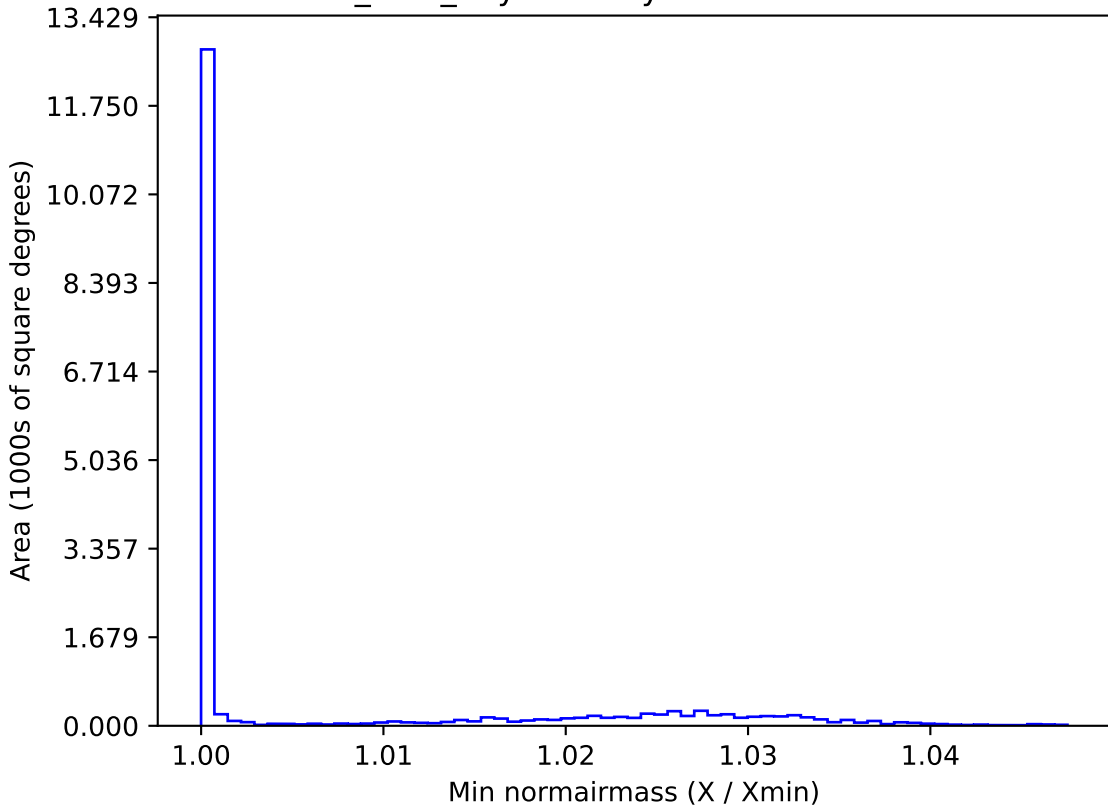
baseline_v3.5_10yrs WFD y band: Min normairmass
