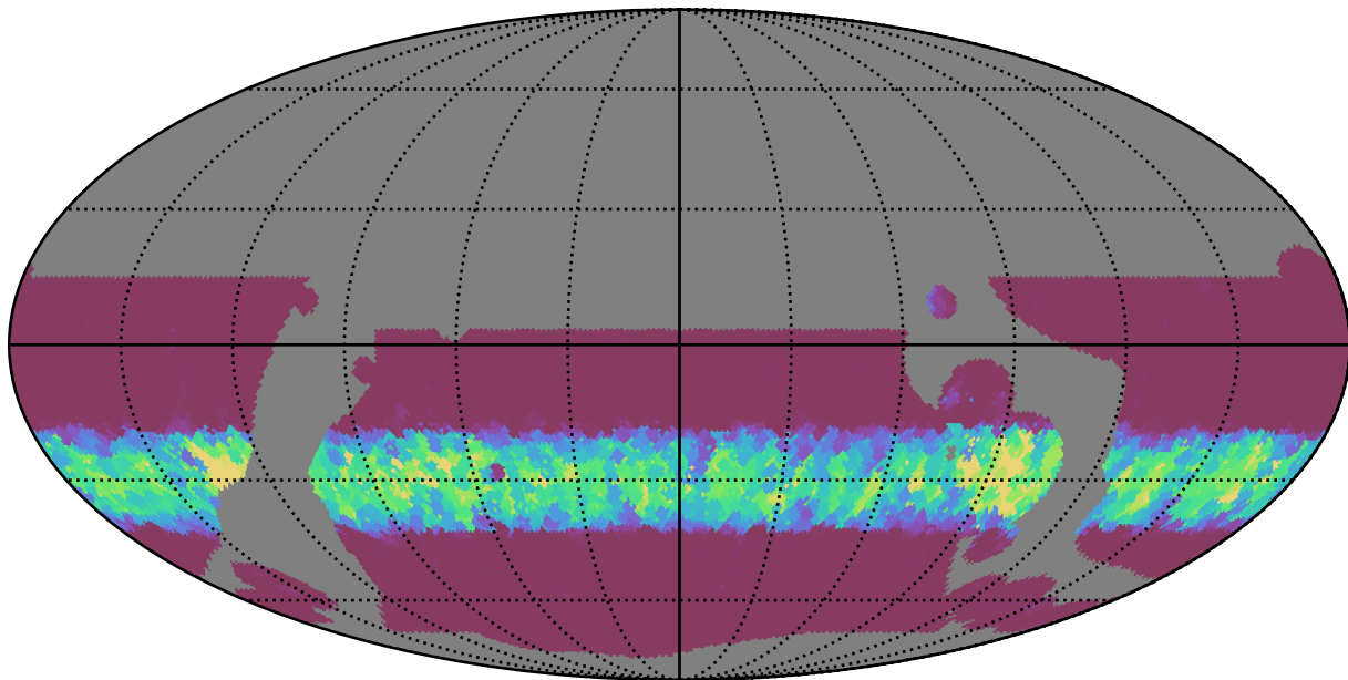
baseline_v3.5_10yrs WFD u band: Min normairmass
