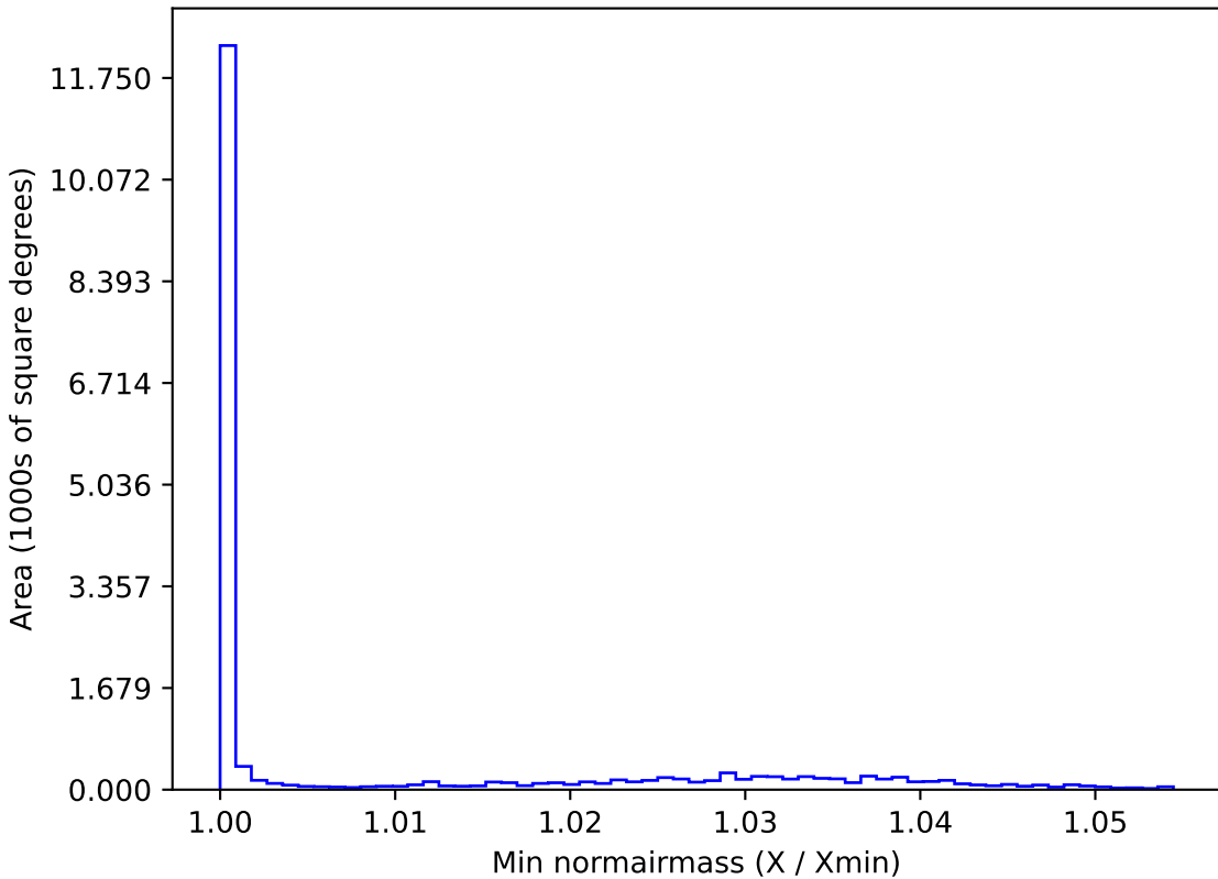
baseline_v3.5_10yrs WFD u band: Min normairmass
