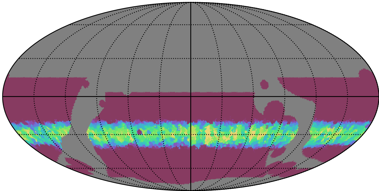
baseline_v3.5_10yrs WFD r band: Min normairmass
