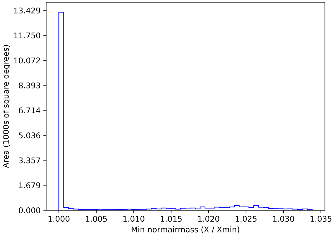
baseline_v3.5_10yrs WFD i band: Min normairmass
