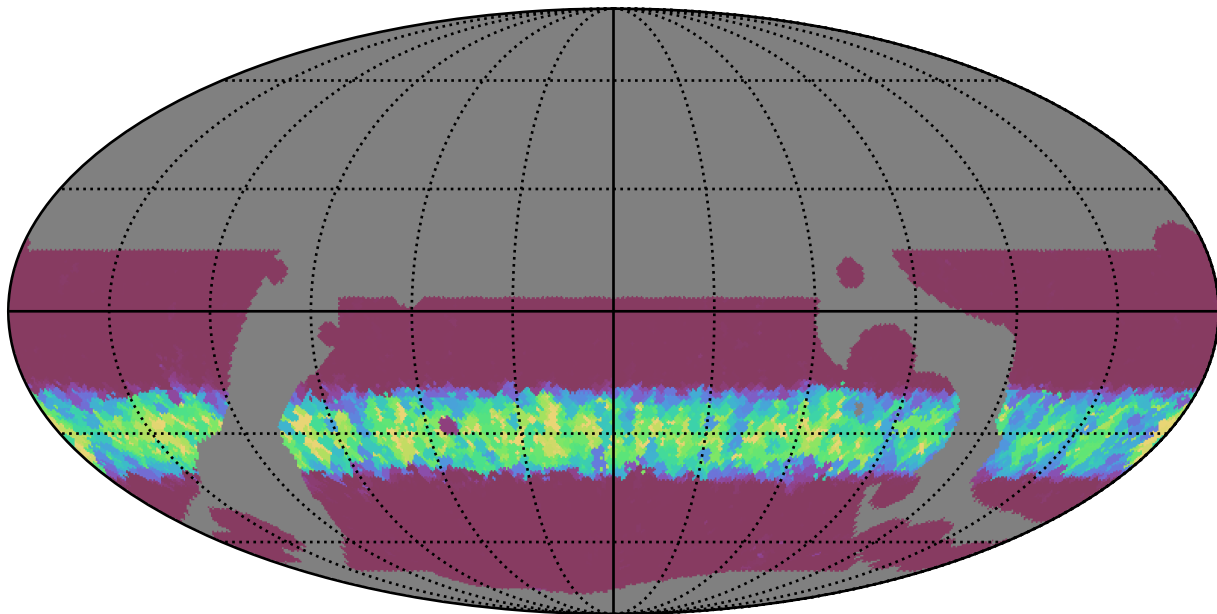
baseline_v3.5_10yrs WFD g band: Min normairmass
