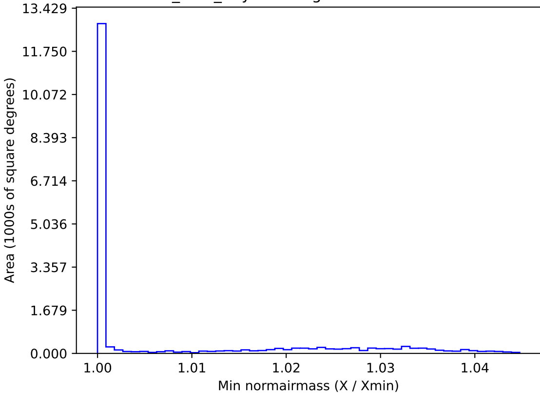
baseline_v3.5_10yrs WFD g band: Min normairmass
