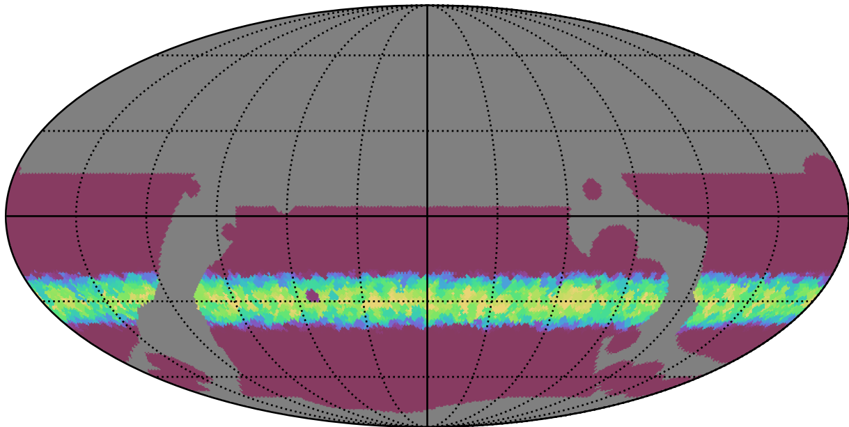
baseline_v3.5_10yrs WFD all bands: Min normairmass
