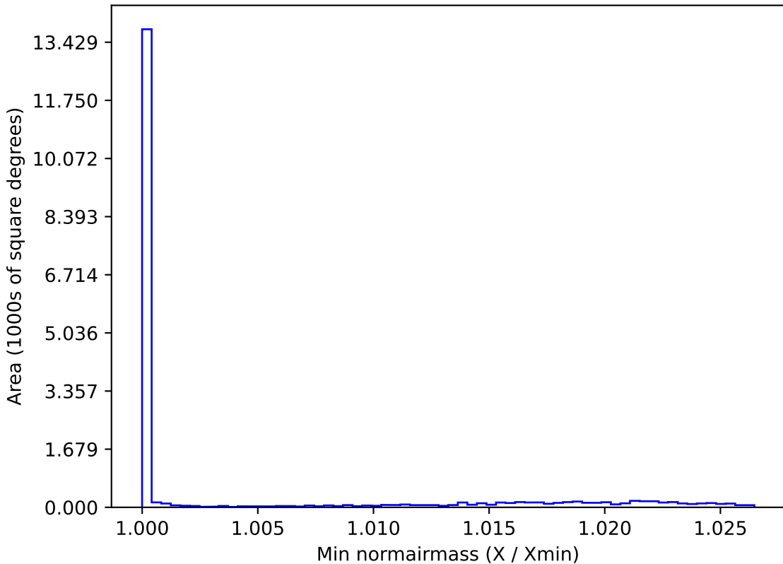
baseline_v3.5_10yrs WFD all bands: Min normairmass
