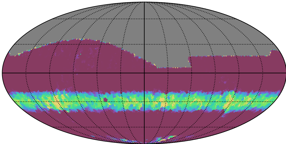
baseline_v3.5_10yrs All sky z band: Min normairmass
