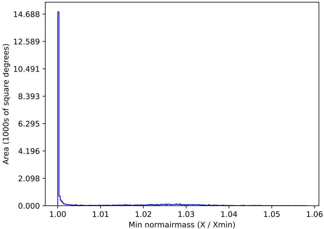
baseline_v3.5_10yrs All sky y band: Min normairmass
