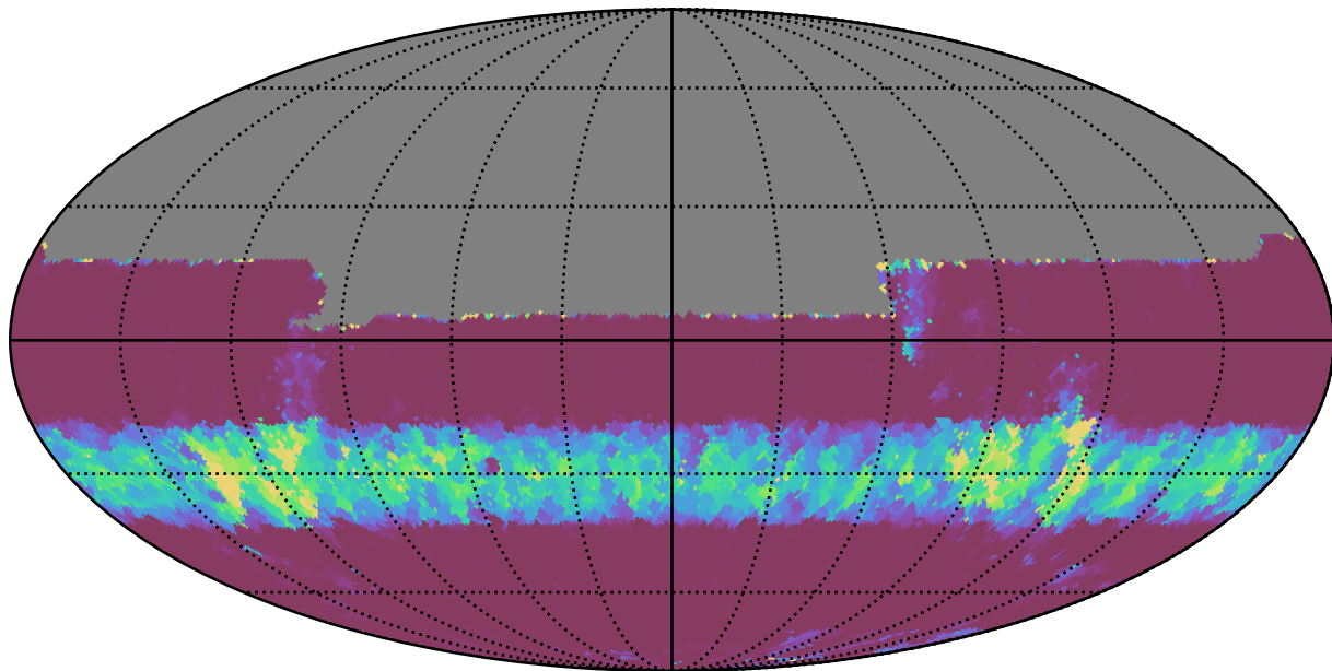
baseline_v3.5_10yrs All sky u band: Min normairmass
