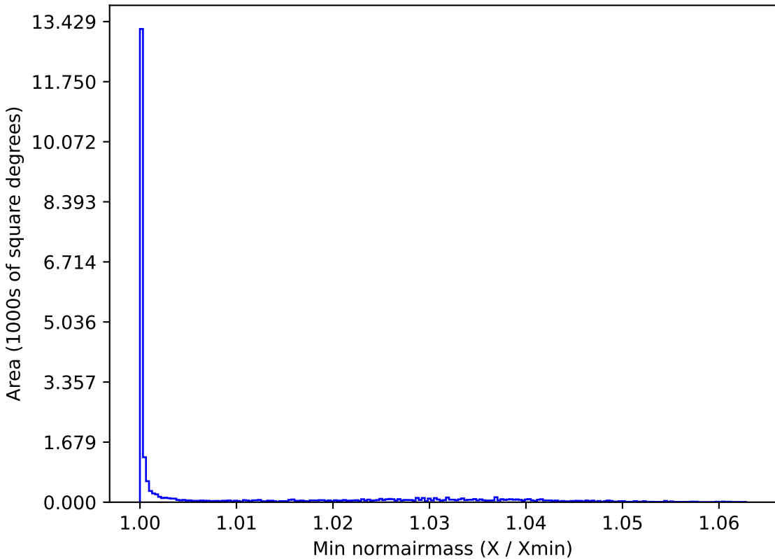
baseline_v3.5_10yrs All sky u band: Min normairmass
