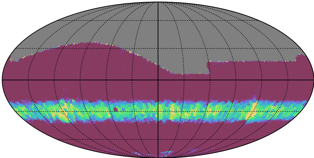
baseline_v3.5_10yrs All sky r band: Min normairmass
