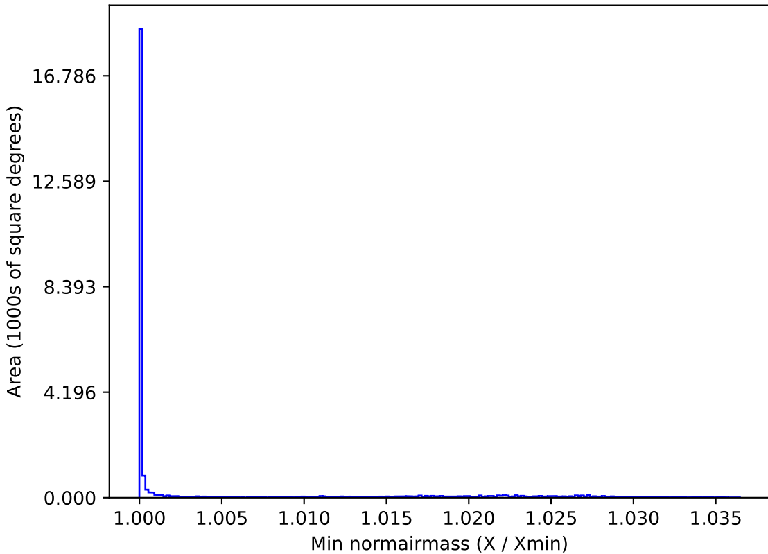
baseline_v3.5_10yrs All sky r band: Min normairmass
