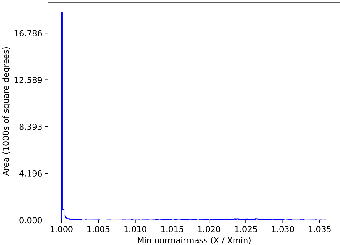
baseline_v3.5_10yrs All sky i band: Min normairmass
