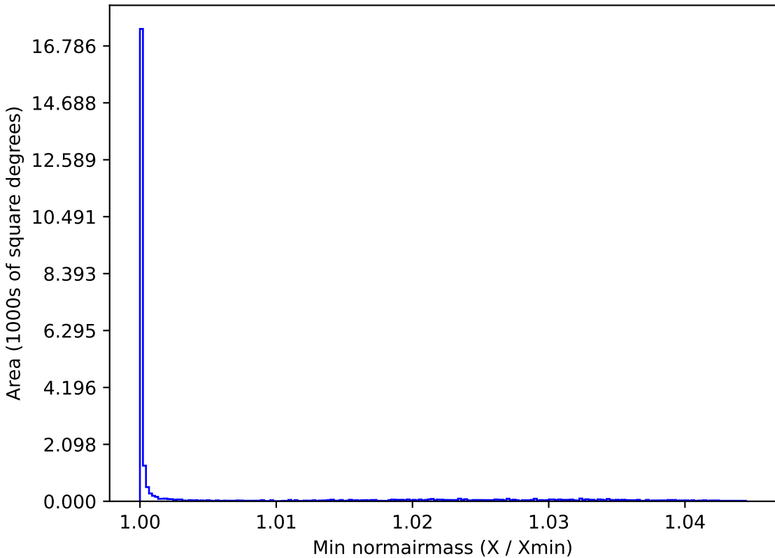
baseline_v3.5_10yrs All sky g band: Min normairmass
